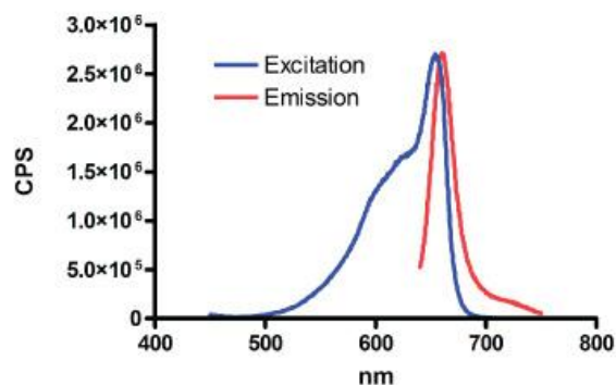
Fluorescence excitation and emission spectra of APC in 100 mM sodium phosphate (pH 7.2) + 1 mM EDTA and 1 mM sodium azide. The emission scan was taken with excitation at 630 nm. The excitation scan was taken with an emission at 660 nm. The curves were normalized to equalize peak heights.
